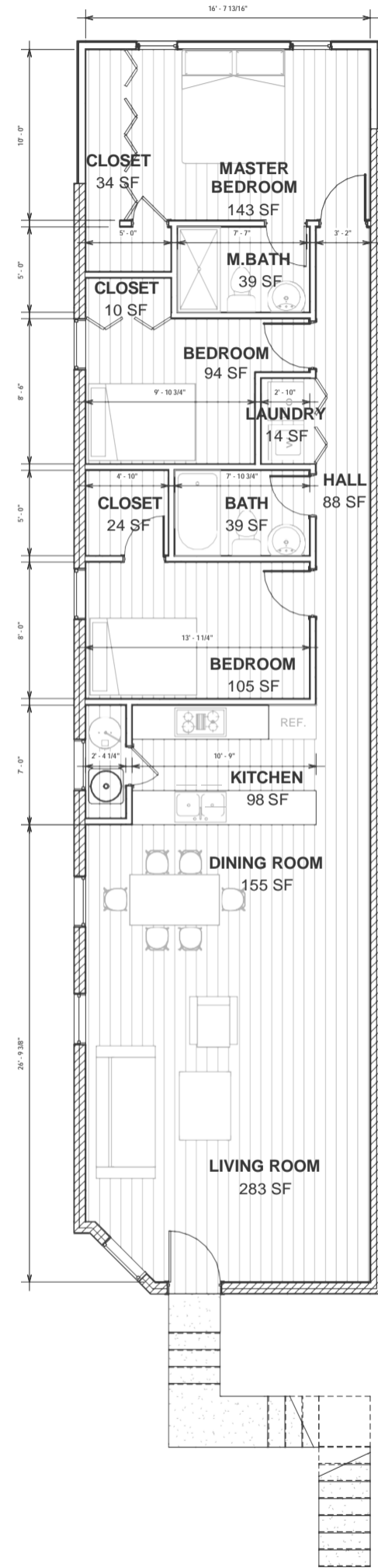
1 BASEMENT FLOOR PLAN UNIT#1 3 16 1 0
